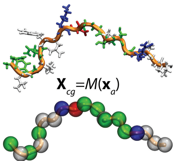
Coarse-graining
